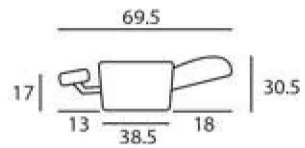
STANDARD Recliner Mechanism
